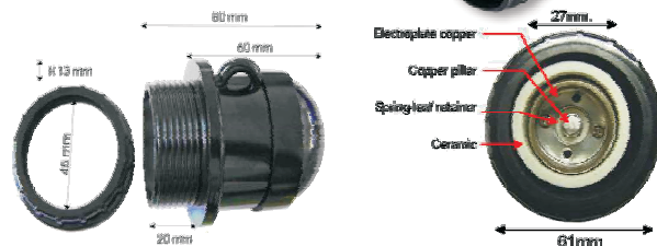
325.024A 電木保温燈頭 (線徑1.25mm/線長3米/温控器) Lamp cord only 10'(1.25mm/3M/with switch)
